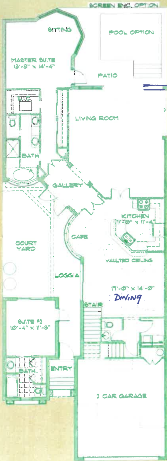
First Floor
